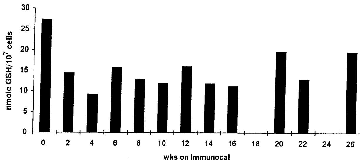
Figure 2. Changes in blood lymphocyte glutathione levels during treatment.
